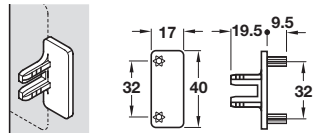
Dowel fixing
